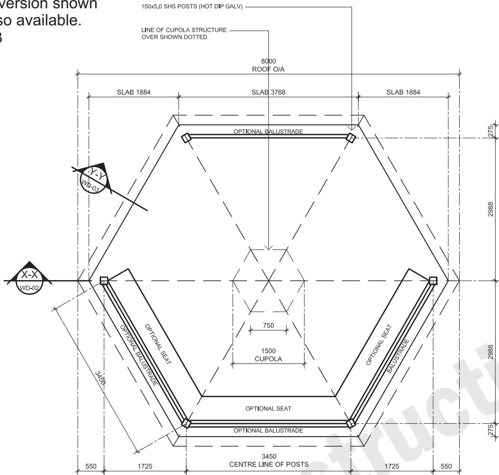
LAYOUT PLAN 1:50 150x150 HDG STEEL POSTS AND CUPOLA OPTION
