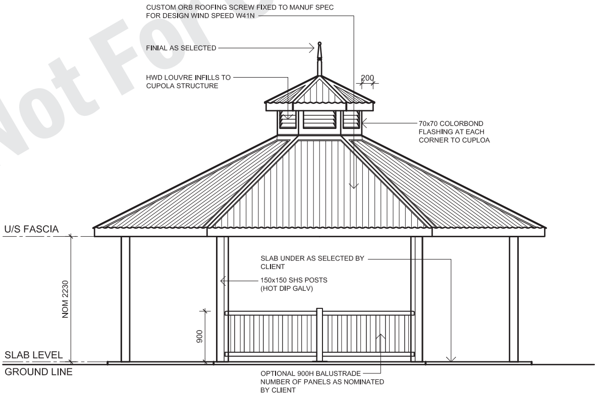
ELEVATION 1:50 150x150 HDG STEEL POSTS AND CUPOLA OPTION
